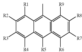
Structural formula (9)
