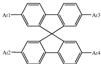
Structural formula (2)
