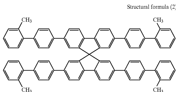
Structural formula (2)
