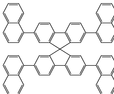
Structural formula (5)
