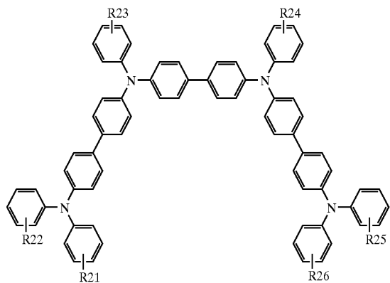
Structural formula (3)
