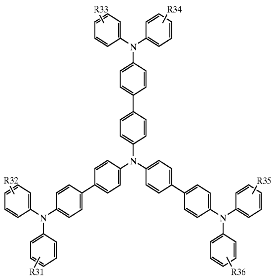
Structural formula (3)
